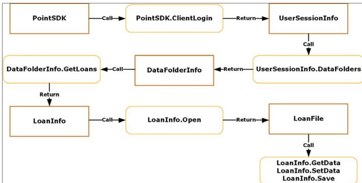
Figure 10: Class Diagram
